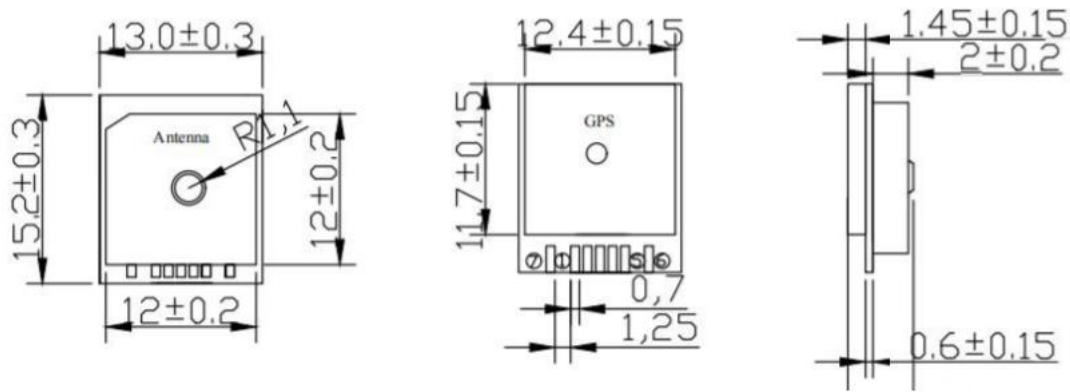
Dimensional Drawing View
